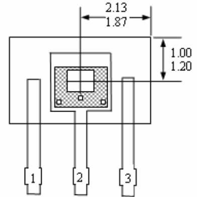
Sensor Location
